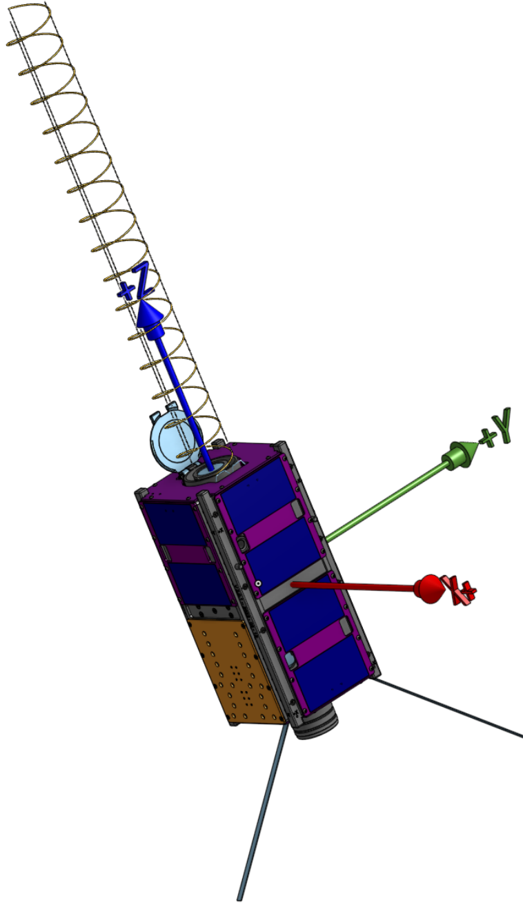
Figure 6.1: OreSat1 axis definition
